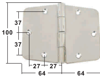
HINGE stamped AISI 316 buff polished
