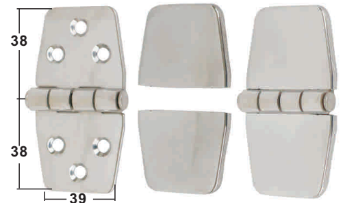
COVERS WITH HINGES AISI 304
