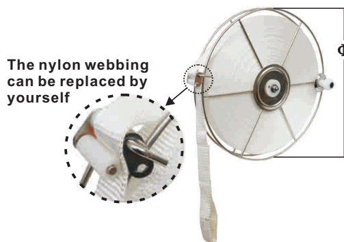
STERN ANCHOR ROLLER AISI 304 mounting for \Phi 22\text{mm} & 25mm rail tube with belt
