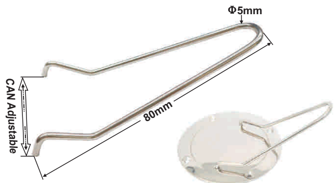
INSPECTION PORT ADJUSTABLE KEY AISI 304 Stainless steel Flexible wire you can use one key for all kind of inspection ports which is the advantage. ITEM NO. B22-001
