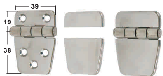
COVERS WITH HINGES AISI 304
