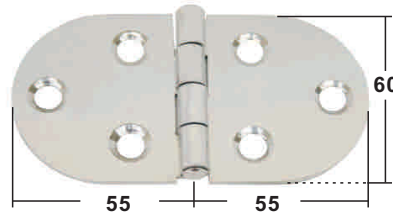
HINGE stamped AISI 304
