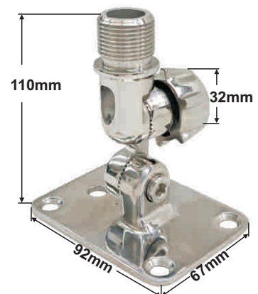
NEW ANTENNA RATCHET MOUNTS casted AISI 316 Thread 1"-14 ITEM NO. B22-019
