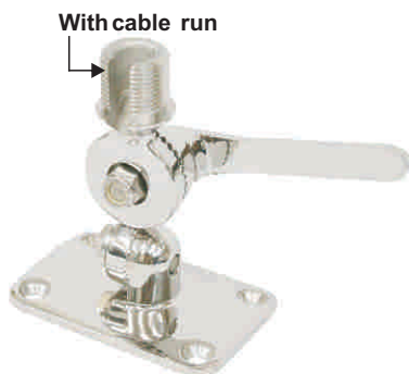
ANTENNA RATCHET MOUNTS casted AISI 316 Socket 4-way ratchet design for mounting versatility. With cable run. ITEM NO. Base Thread Weight 009896 2-1/4"x3-1/2" 1"-14 640g economic
