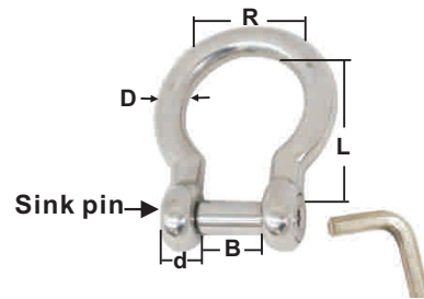
BOW SHACKLES WITH OVAL SINK PIN AISI 316
