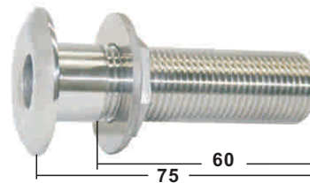
SKIN FITTING casted AISI 316 ITEM NO. Size Thread Weight/g 030012 1/2" BSP 140 030034 3/4" BSP
