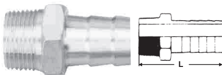
HOSE NIPPLES (HONP) Threaded type: DIN 2999, NPT ITEM NO. SIZE L PACKING MATERIAL 300034 3/4 72.86 150/Box AISI 316 300001 1 82.46 80/Box AISI 316
