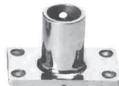
60° RECTANGULAR BASE casted AISI 316 ITEM NO. Tube O.D. Base mm Weight/g 009617 32mm(1-1/4") 82x42 250
