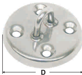
SWIVEL BASE stamped AISI 304 ITEM NO. Dmm Weight/g 005061 55 40
