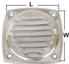
VENT stamped AISI 304 ITEM NO. L mm W mm Thickness Weight B19-029 100 100 1 mm 70g
