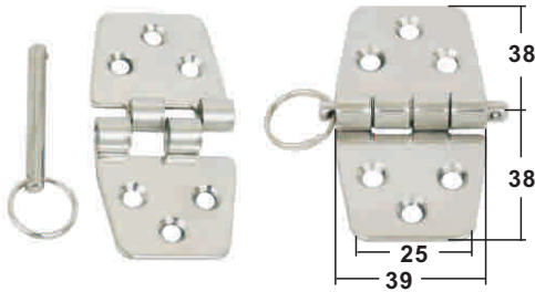
HINGE WITH PIN stamped AISI 304
