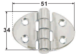
HINGE Stamped AISI 316
